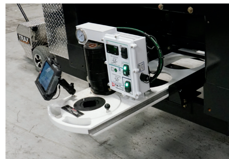
TM-7 HD Plus valve operator provides 2500 ft-lb of torque for turning large valves
